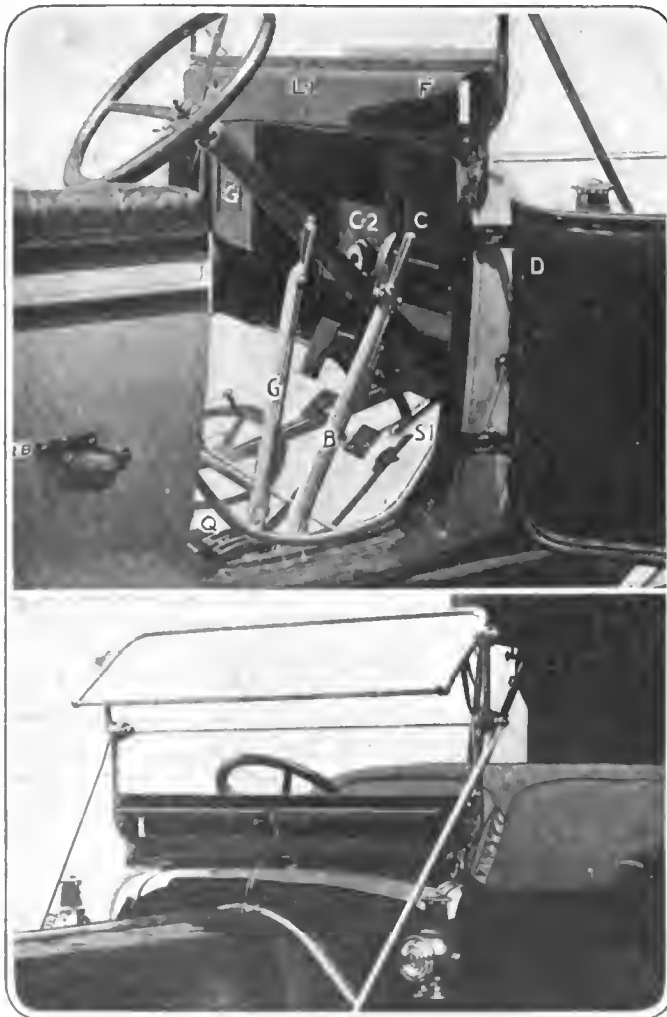
Fig. 2—All doors are made to open, showing how the levers are placed entirely within the body. The new ventilator can also be seen Fig. 3—Showing the new type of windshield, the open flaps of the ventilator and the neat side lamps
